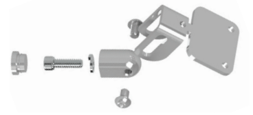
Post-Side Handrail Bracket
